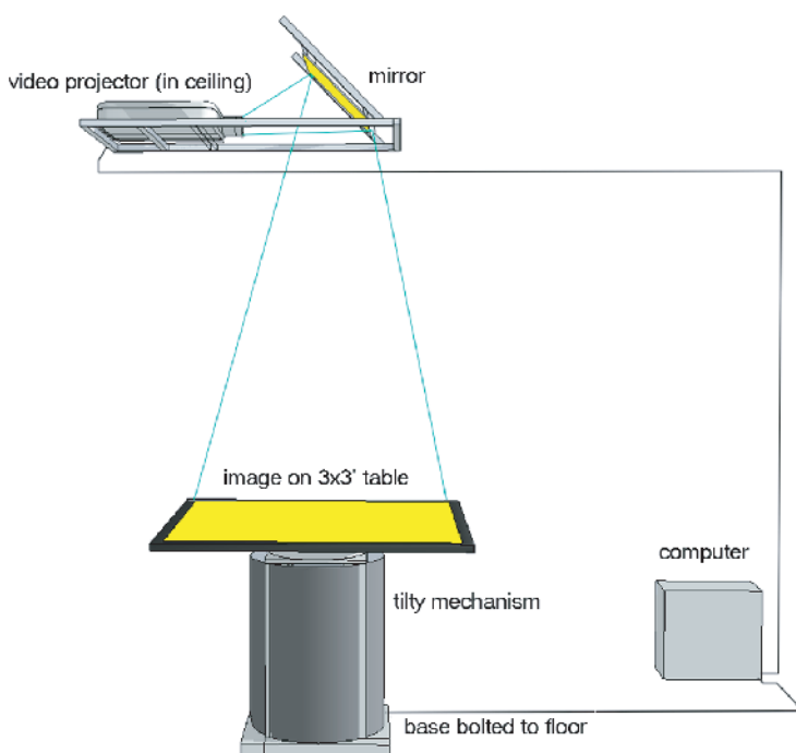
Example of acoustic tile ceiling mount design
